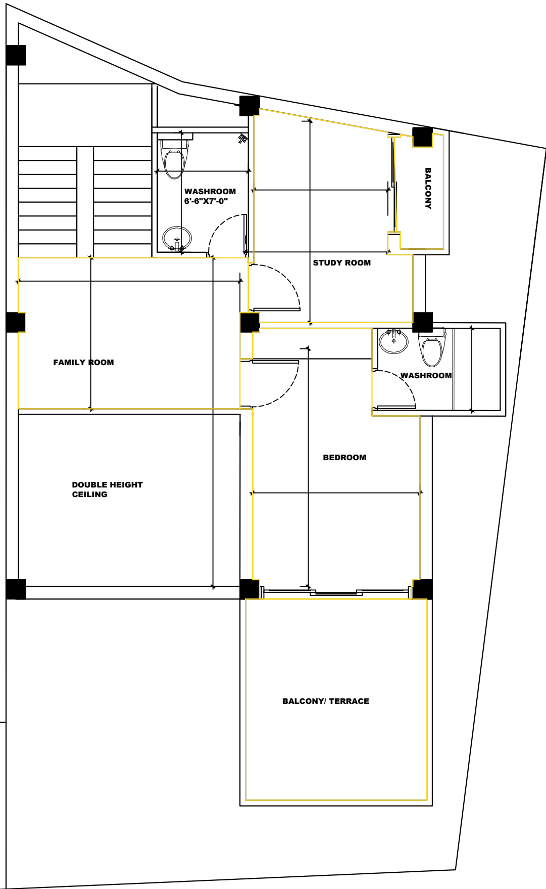
FIRST FLOOR PLAN AREA= 830 sq. ft
